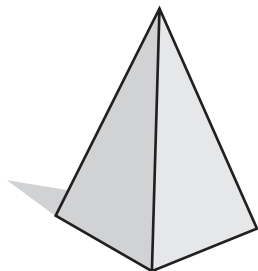
triangular pyramid
